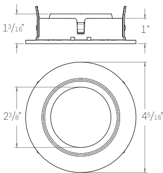
ED3-RFST ROUND FIXED STANDARD TRIM
