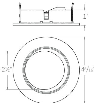
ED3-RAST ROUND ADJUSTABLE STANDARD TRIM Adjustable trim styles for use with adjustable AIC and ANC models only.
