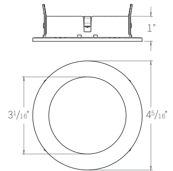
ED3-RFWL ROUND FIXED WET LOCATION
