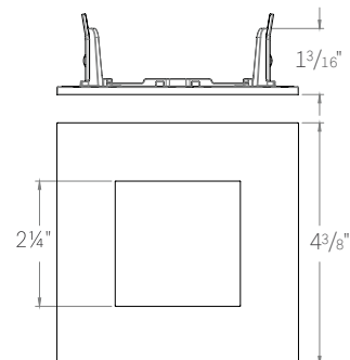
ED3-SFWL SQUARE FIXED WET LOCATION
