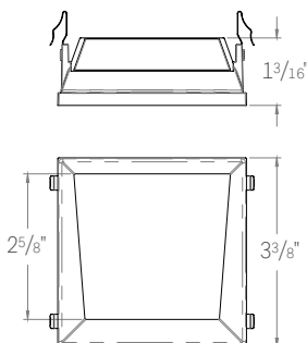
ED3-SATL SQUARE ADJUSTABLE TRIMLESS Adjustable trim styles for use with adjustable AIC and ANC models only.
