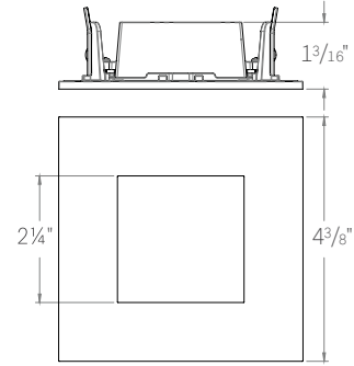
ED3-SFWW SQUARE FIXED WALL WASH
