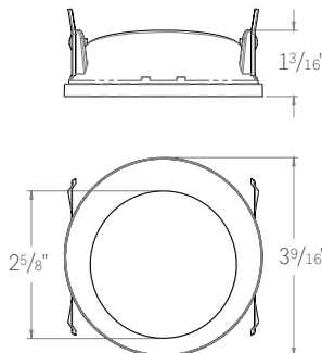
ED3-RATL ROUND ADJUSTABLE TRIMLESS Adjustable trim styles for use with adjustable AIC and ANC models only.
