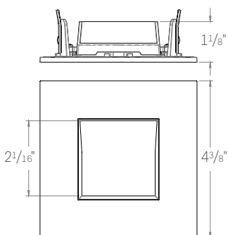
ED3-SAST SQUARE ADJUSTABLE STANDARD TRIM Adjustable trim styles for use with adjustable AIC and ANC models only.
