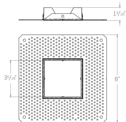
ED3-S-TL SQUARE TRIMLESS MUDPLATE For use with AIC, ANC, SNIC housings only
