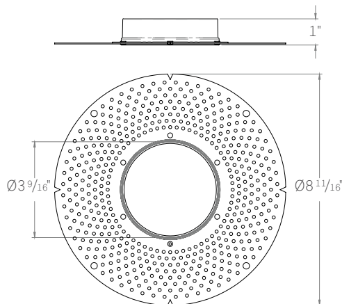
ED3-R-TL ROUND TRIMLESS MUDPLATE For use with AIC, ANC, SNIC housings only
