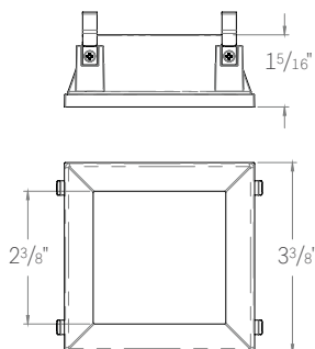
ED3-SFTL SQUARE FIXED TRIMLESS
