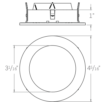
ED3-RFWW ROUND FIXED WALL WASH
